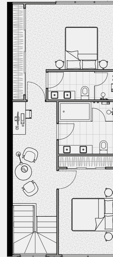
SECOND FLOOR
