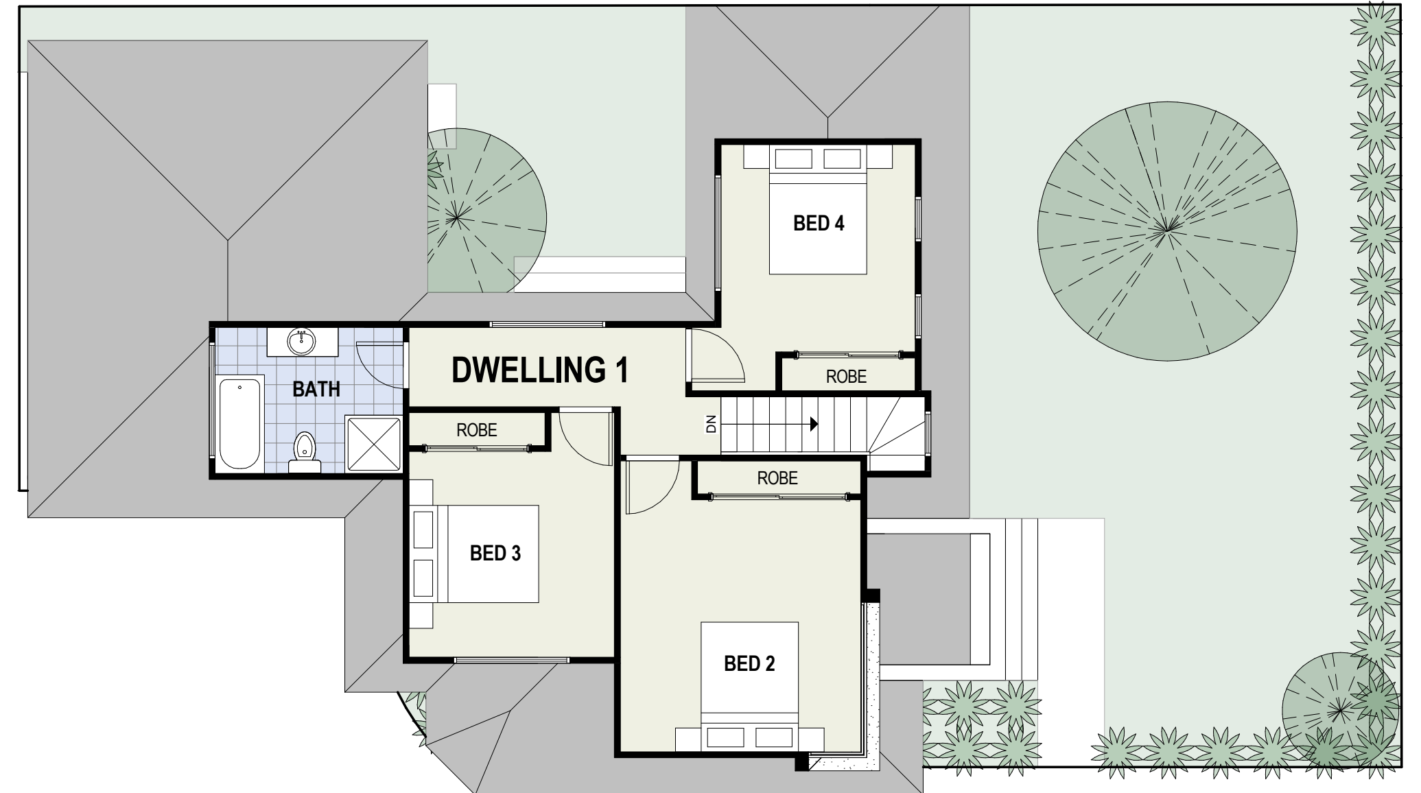
FIRST FLOOR
