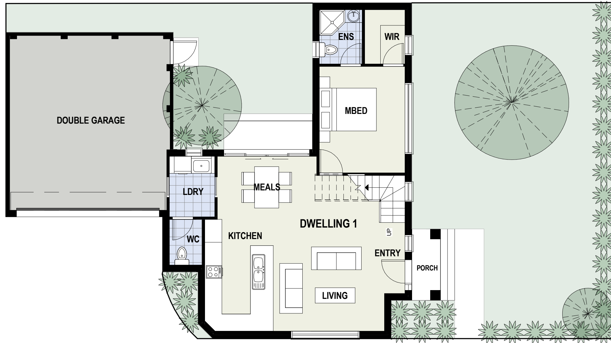
GROUND FLOOR
